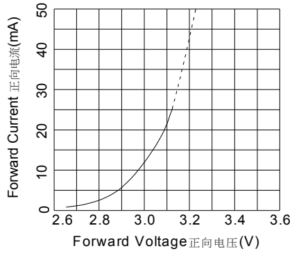
Volt-Ampere Characteristics VF-IF曲线
