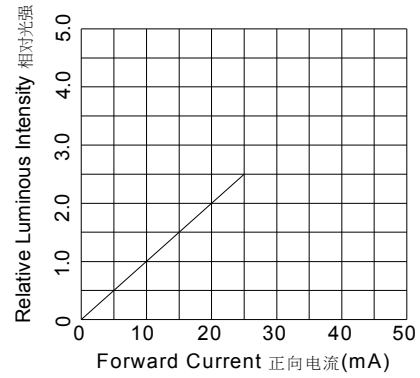
Forward Current VS. Relative Intensity IF-IV曲线
