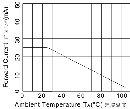
Ambient Temperature VS. Forward Current Ta-IF曲线
